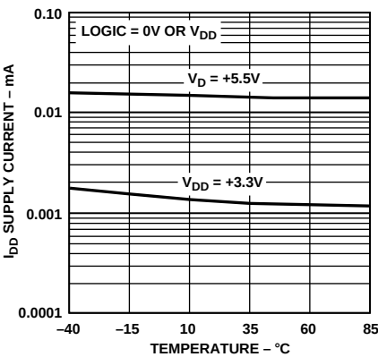
Figure 25. Supply Current vs. Temperature I_{DD}
