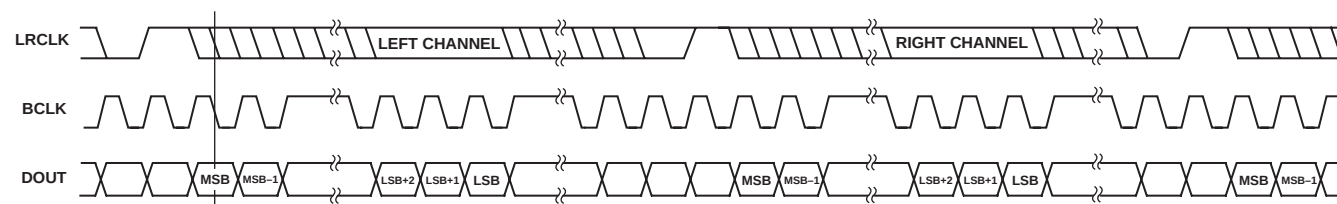
Figure 15. DSP Mode
