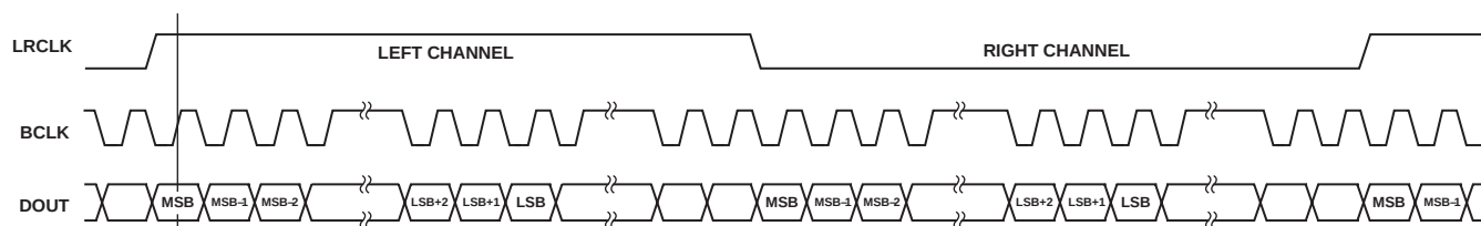
Figure 13. Left-Justified Mode
