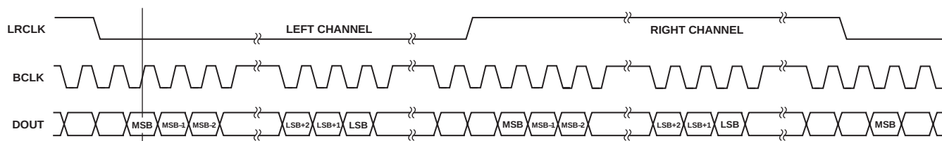
Figure 12. I 2 S Mode
