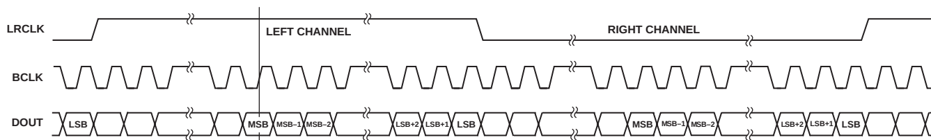
Figure 14. Right-Justified Mode
