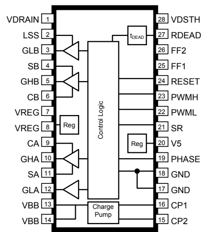
Pinout Diagram
