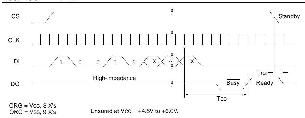
FIGURE 3-8: ERAL
