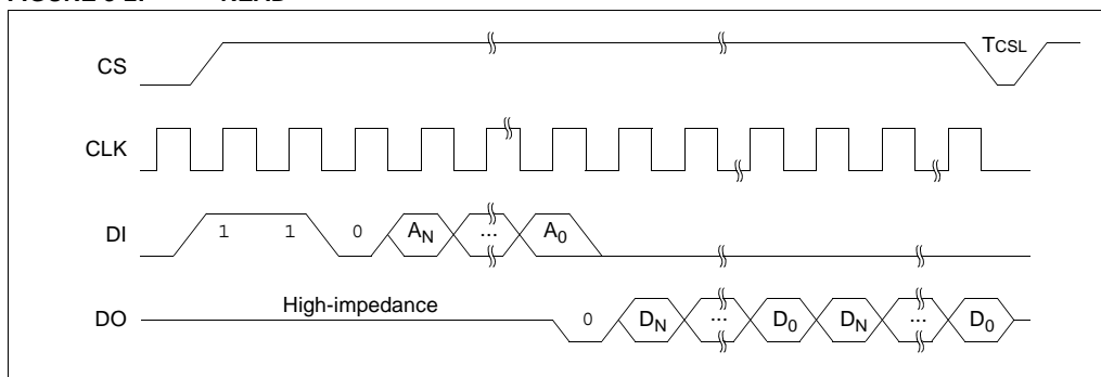
FIGURE 3-2: READ
