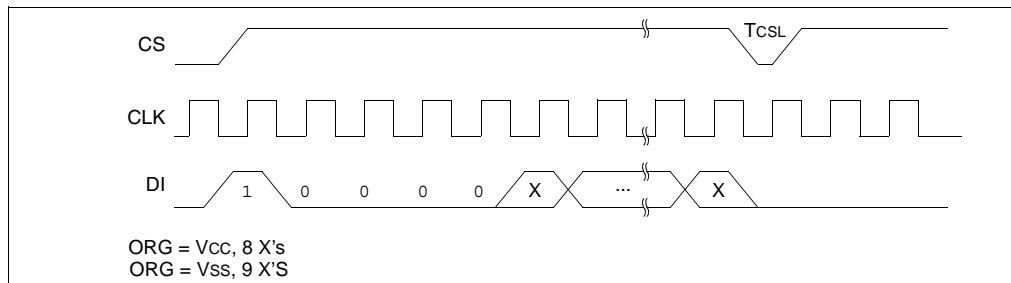
FIGURE 3-5: WRITE
