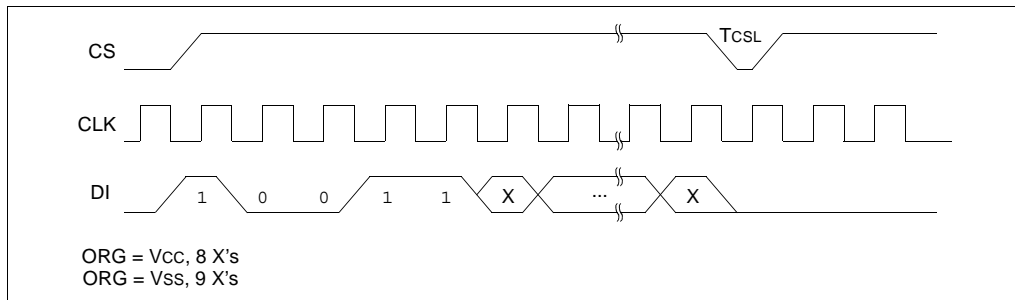
FIGURE 3-3: EWEN
