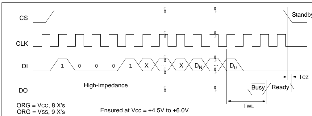
FIGURE 3-6: WRAL
