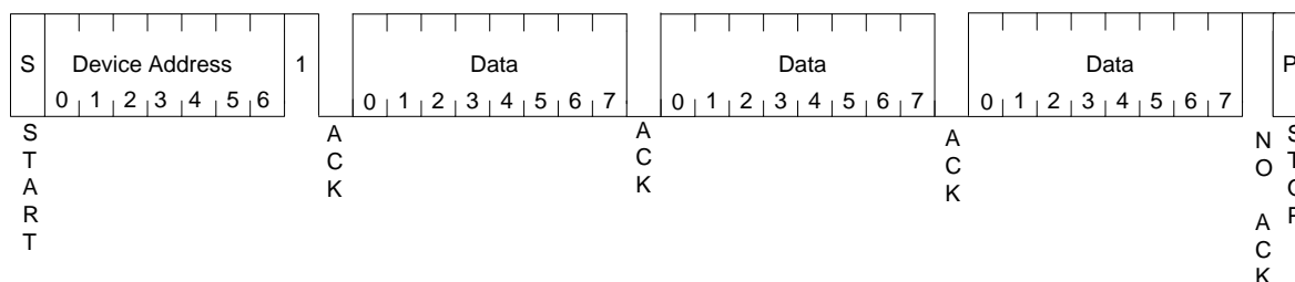
Figure 36. Read Operation
