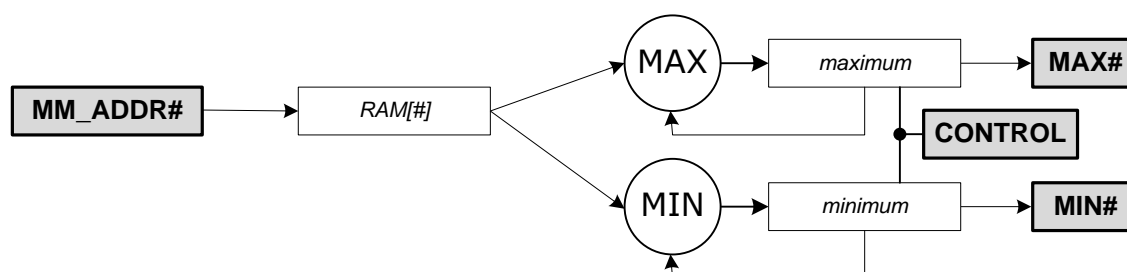
Figure 23. Min/Max Tracking
