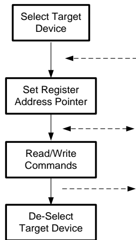
Figure 28. SSI Protocol
