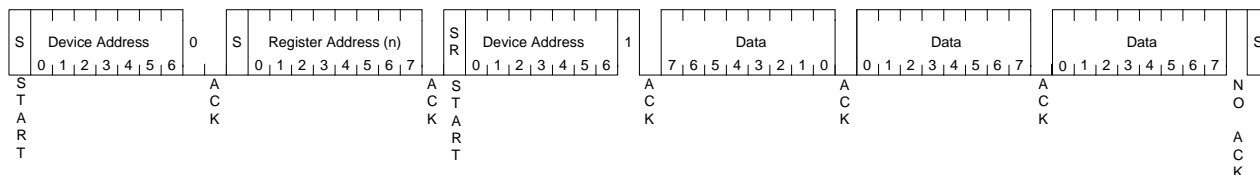
Figure 38. Reading Multiple Registers
