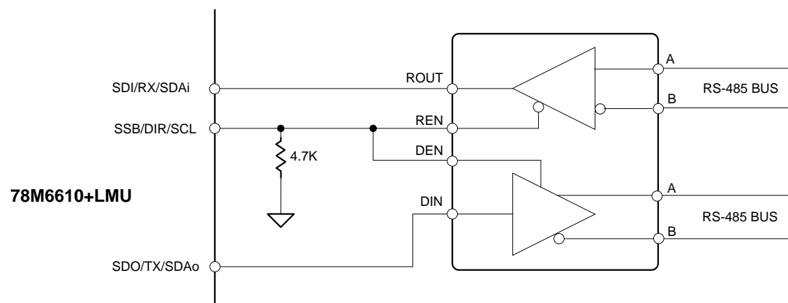
Figure 26. RS-485 Interface
