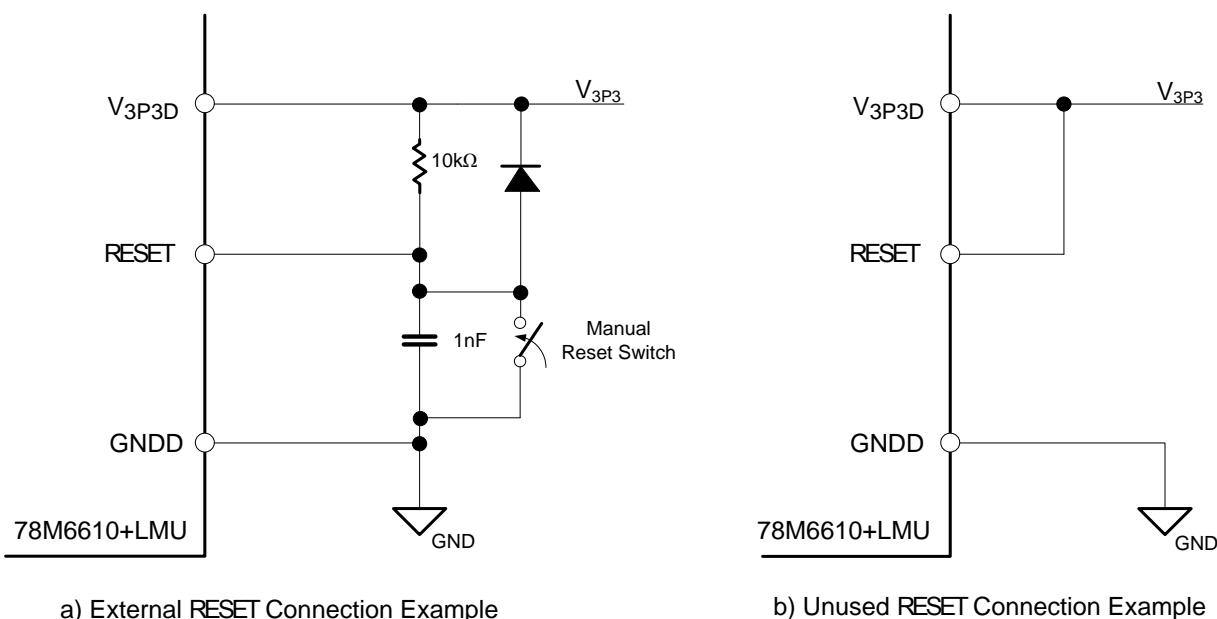
Figure 6. Reset Connections
