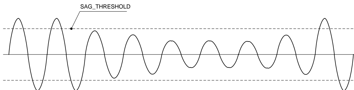
Figure 24. Voltage Sag
