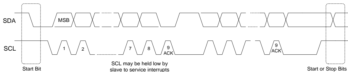
Figure 32. I²C Bus Characteristics
