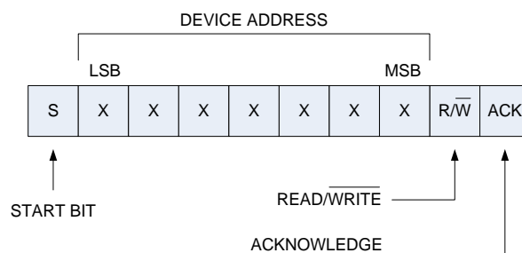
Figure 33. I²C Device Addressing
