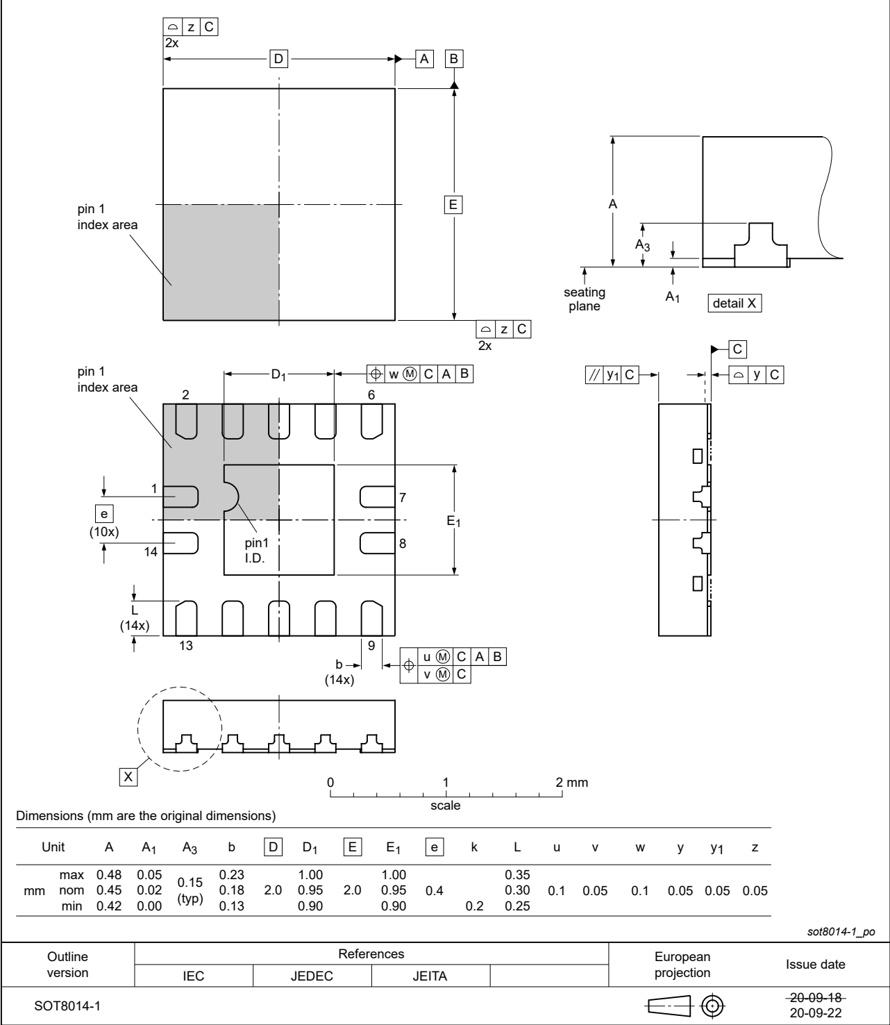
Fig. 17. Package outline SOT8014-1 (DHXQFN14)
