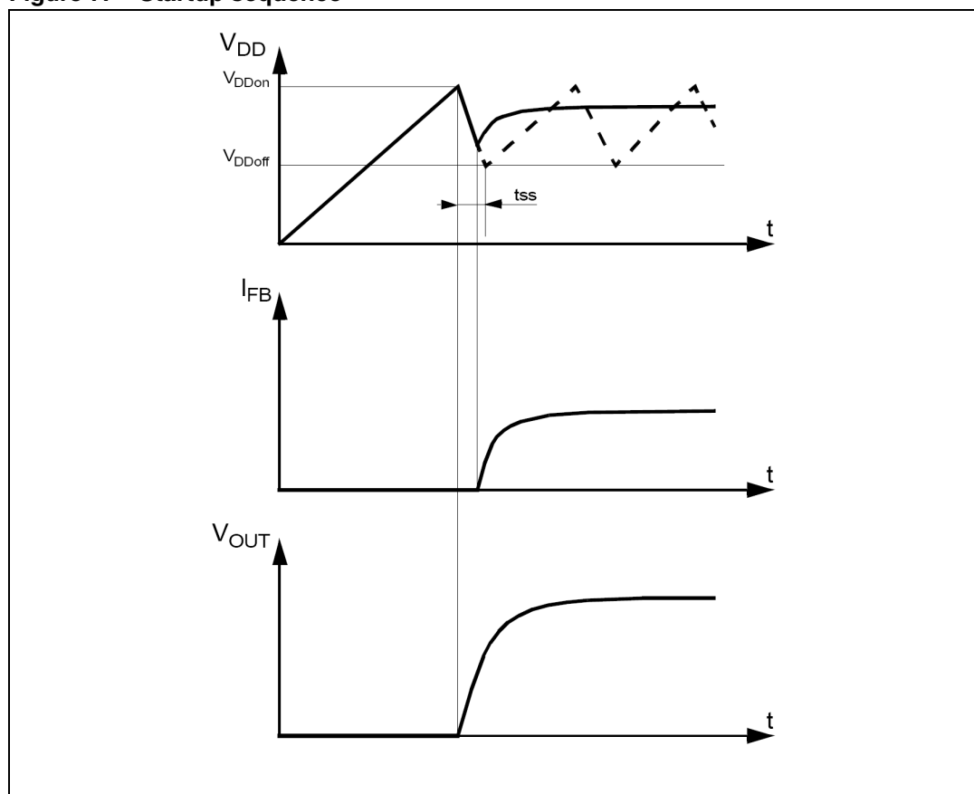
Figure 7. Startup sequence
