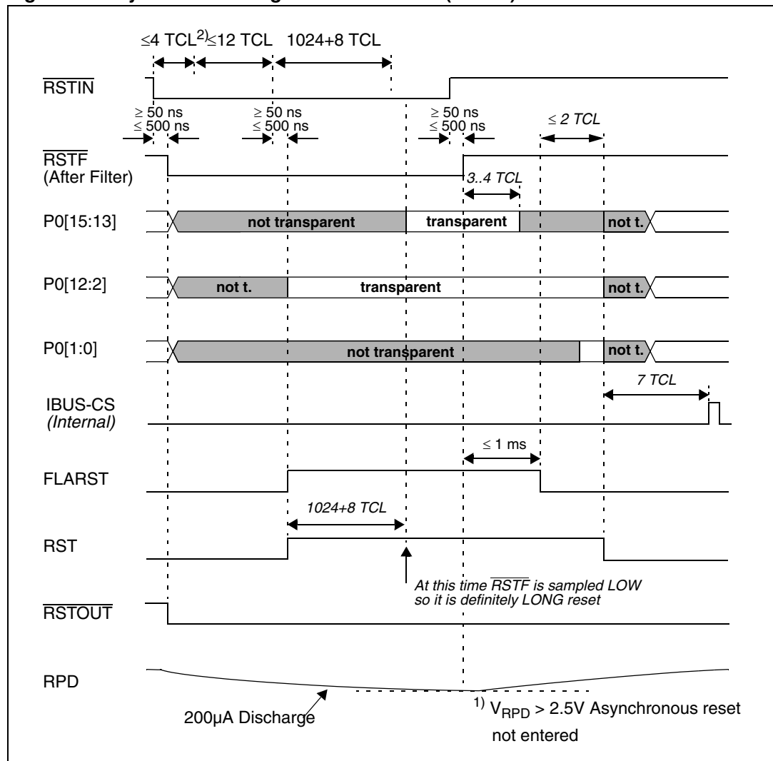
Figure 24. Synchronous long hardware RESET ( \overline{\text{EA}} = 1 )
