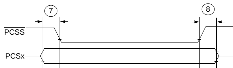
Figure 38. DSPI PCS strobe ( \overline{\text{PCSS}} ) timing
