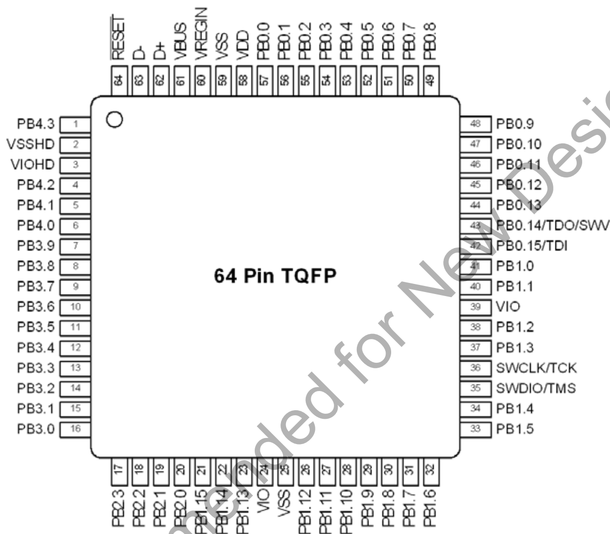
Figure 6.3. SiM3U1x6-QQ Pinout
