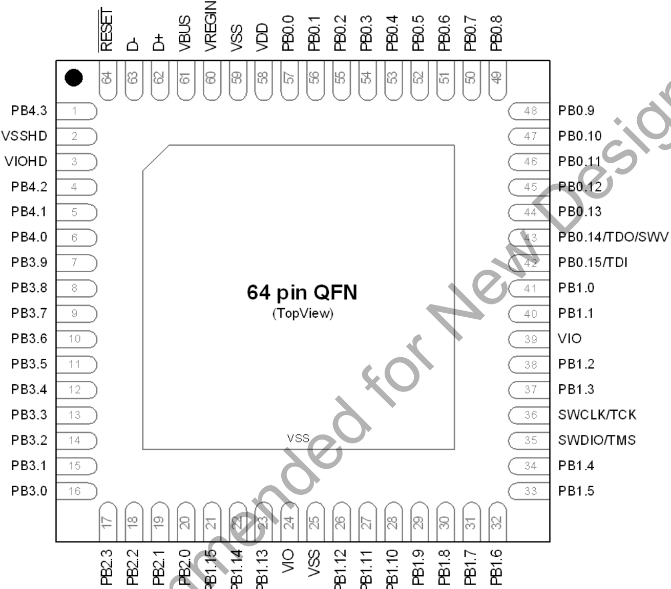
Figure 6.4. SiM3U1x6-GM Pinout
