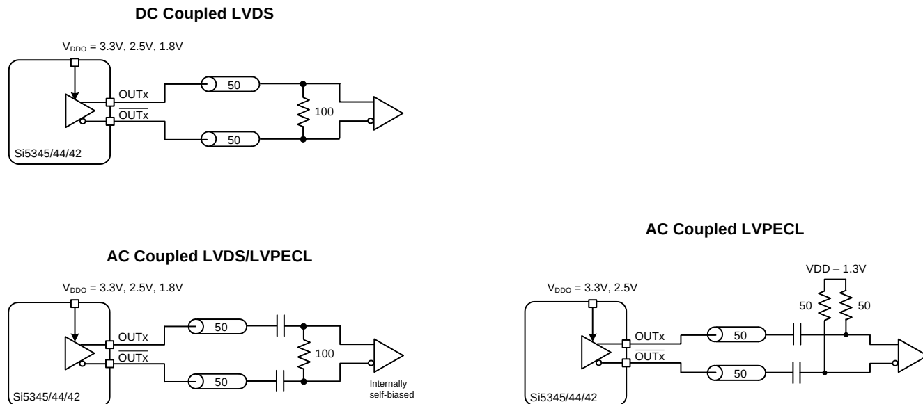
Figure 19. Supported Differential Output Terminations
