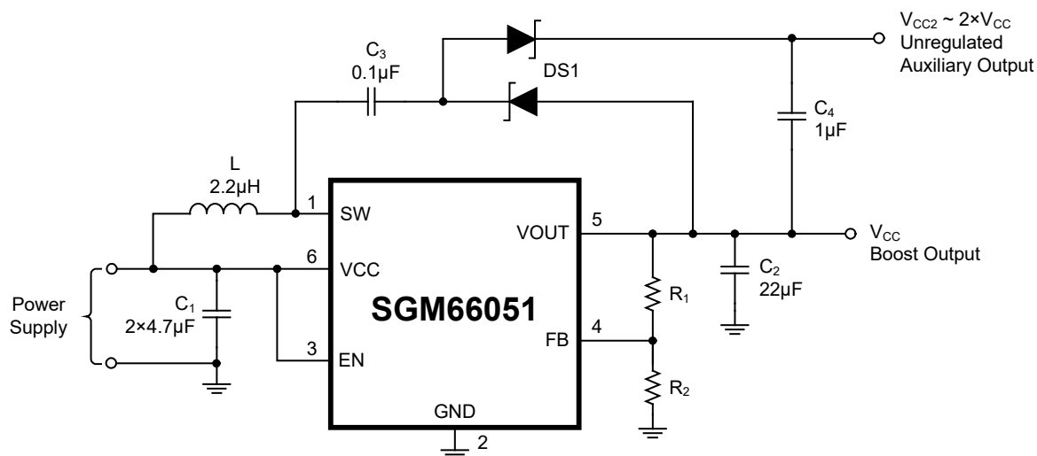
Figure 3. Supply with an Auxiliary Positive Output
