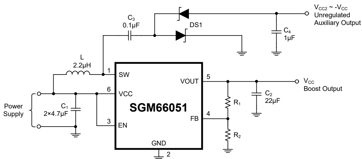
Figure 4. Supply with an Auxiliary Negative Output
