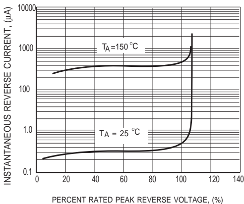
FIG.2 MAXIMUM REVERSE CHARACTERISTICS
