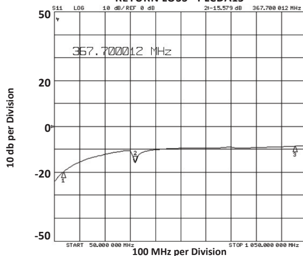
FIGURE 6 RETURN LOSS - PLCDA15
