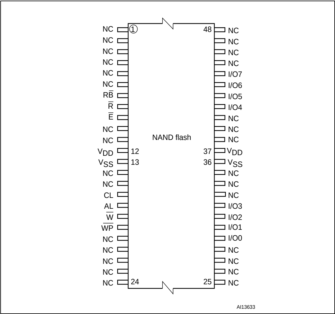
Figure 3. TSOP48 connections
