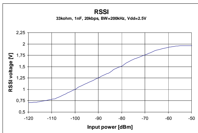
Figure 10. RSSI Voltage
