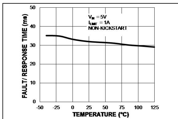
FIGURE 2-7: FAULT/ Response Time vs. Temperature.
