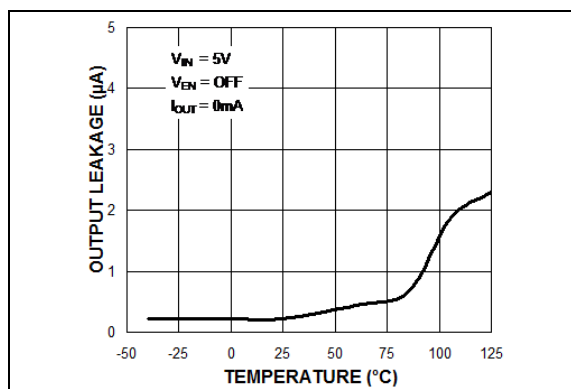
FIGURE 2-10: Output Leakage Current vs. Temperature.
