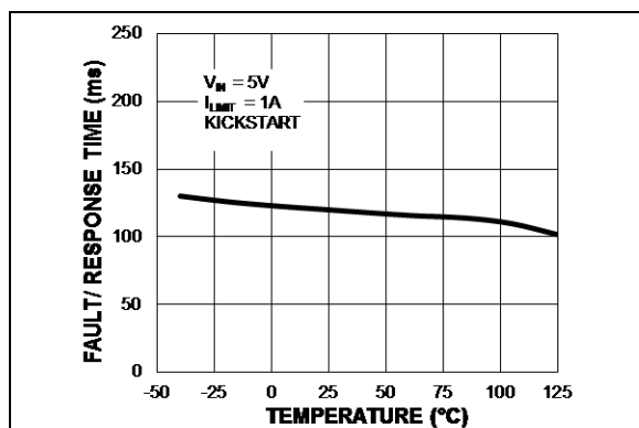
FIGURE 2-8: FAULT/ Response Time vs. Temperature.
