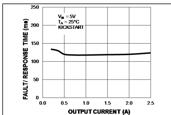
FIGURE 2-9: FAULT/ Response Time vs. Output Current.
