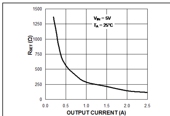
FIGURE 2-12: Current Limit Set Resistor vs. Output Current.
