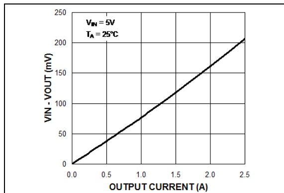
FIGURE 2-11: V_{IN} - V_{OUT} vs. Output Current.
