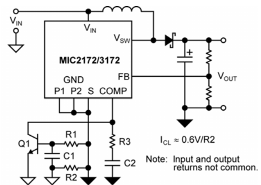
Figure 9. Current Limit
