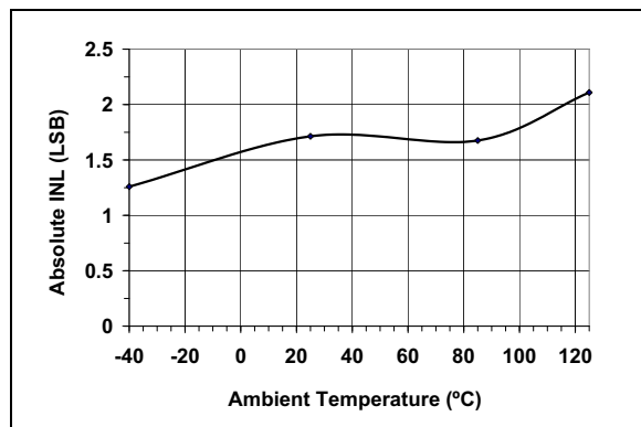
FIGURE 2-7: Absolute INL vs. Temperature (MCP4922).
