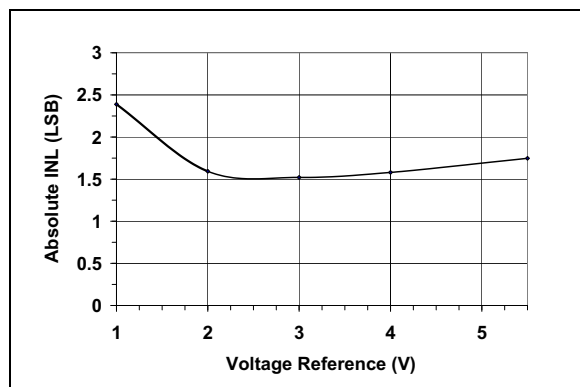
FIGURE 2-8: Absolute INL vs. V_{REF} (MCP4922).
