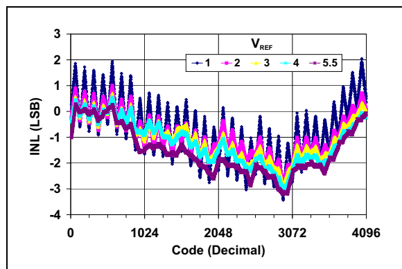
FIGURE 2-9: INL vs. Code and V_{REF} (MCP4922).
