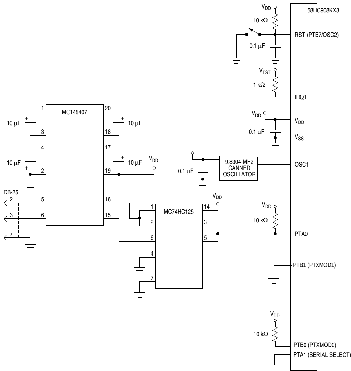
Figure 16-9. Normal Monitor Mode Circuit
