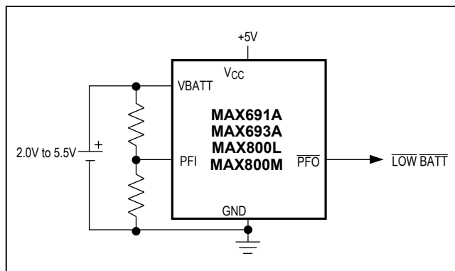
Figure 7. Low-Battery Indicator
