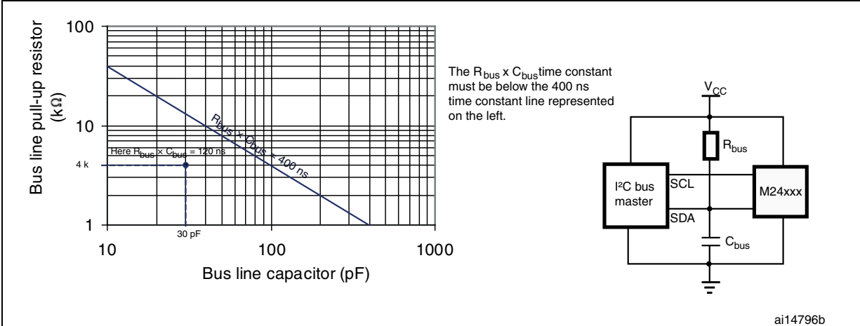
Figure 3. I 2 C Fast mode ( f_C = 400 kHz): maximum R_{bus} value vs. bus parasitic capacitance ( C_{bus} )
