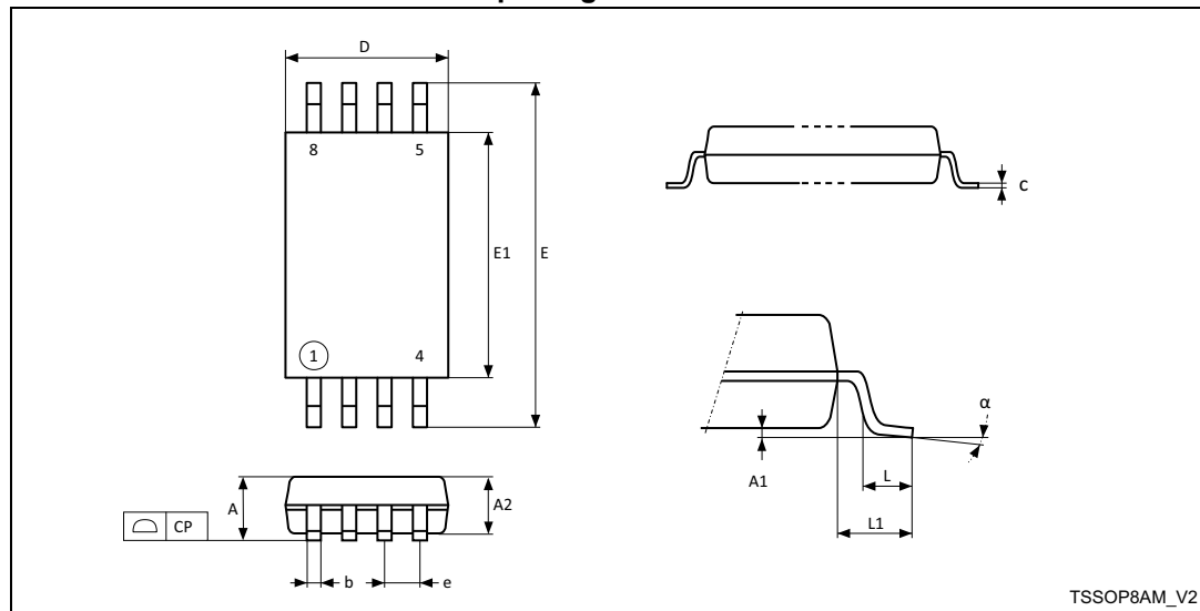
Figure 90. TSSOP8 – 8-lead thin shrink small outline, 3 × 6.4 mm, 0.65 mm pitch, package outline
