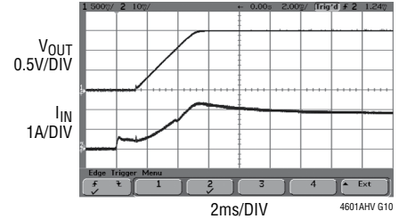
Start-Up, I_{OUT} = 12\text{A} (Resistive Load)
