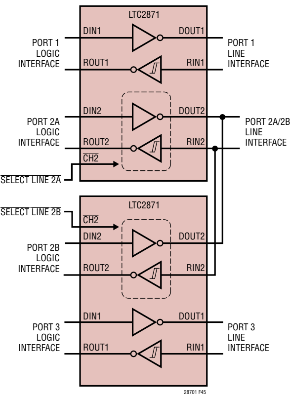
Figure 48. RS232 Triple Transceiver with Selectable Logic Interface
