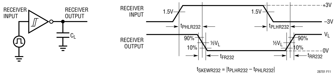
Figure 11. RS232 Receiver Timing Measurements
