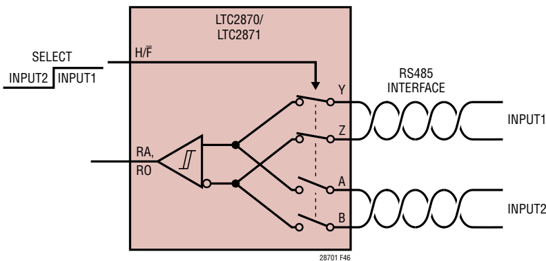
Figure 49. RS485 Receiver with Multiplexed Inputs
