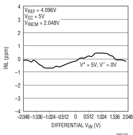
Figure 16. Linearity vs V_{\text{IN}}
