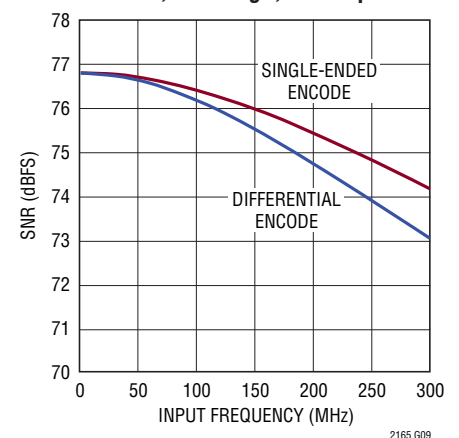
LTC2165 SNR vs Input Frequency, -1dBFS, 2V Range, 125Msps
