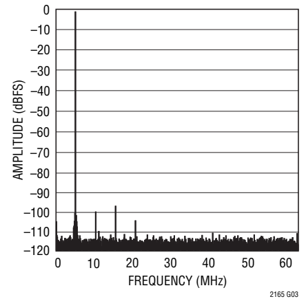
LTC2165 64k Point FFT, f_{IN} = 5\text{MHz} , -1dBFS, 125Msps
