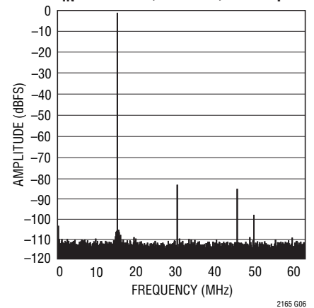
LTC2165 64k Point FFT, f_{IN} = 140\text{MHz} , -1dBFS, 125Msps
