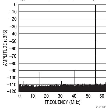
LTC2165 64k Point FFT, f_{IN} = 70\text{MHz} , -1dBFS, 125Msps
