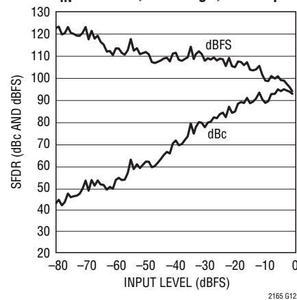
LTC2165 SFDR vs Input Level, f_{IN} = 70\text{MHz} , 2V Range, 125Mps
