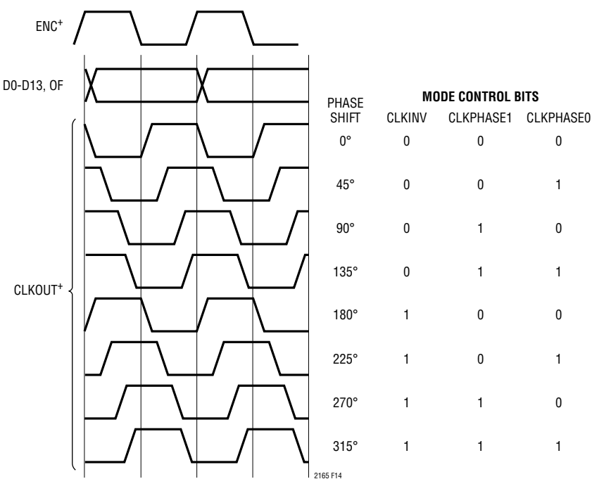
Figure 14. Phase-Shifting CLKOUT
