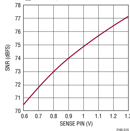
LTC2165 SNR vs SENSE, f_{IN} = 5\text{MHz} , -1dBFS
