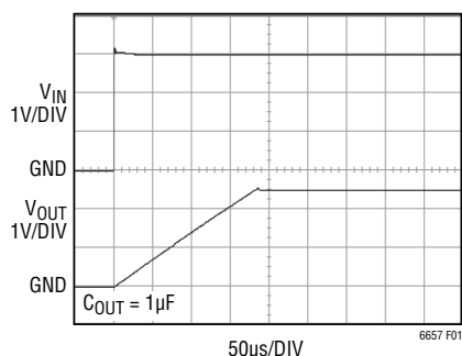
Figure 1. 2.5V Turn-On Characteristics
