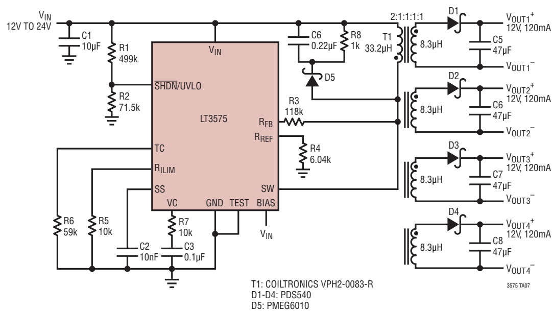
Four Output 12V Isolated Flyback Converter
