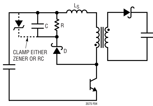
Figure 4. Snubber Clamping
