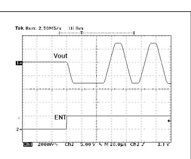
Figure 20. 22KHz Tone
