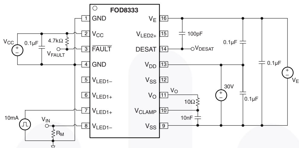
Figure 48. DESAT Sense Delay ( t_{\text{DESAT}(90\%)} ), t_{\text{DESAT}(10\%)} , t_{\text{DESAT}(LOW)} ), DESAT Sense to Low Level FAULT Signal Delay ( t_{\text{DESAT}(FAULT)} ), DESAT Input Mute ( t_{\text{DESAT}(MUTE)} ) Test Circuit
