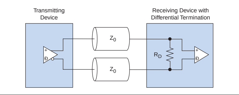
Figure 2–71. LVDS Input Differential On-Chip Termination
