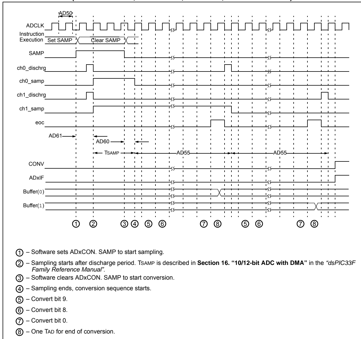
FIGURE 26-28: ADC CONVERSION (10-BIT MODE) TIMING CHARACTERISTICS (CHPS<1:0> = 01, SIMSAM = 0, ASAM = 0, SSRCS<2:0> = 000)
