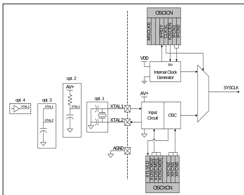
Figure 14.1. Oscillator Diagram
