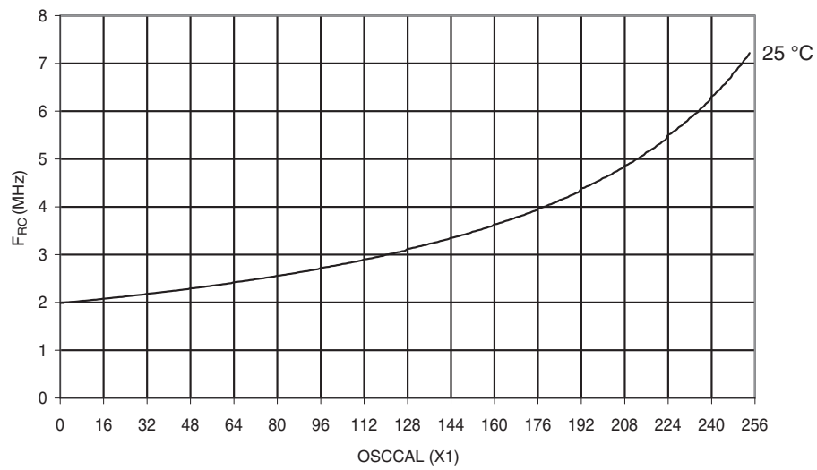
Figure 28-42. Calibrated 4MHz RC Oscillator Frequency vs. Oscal Value
