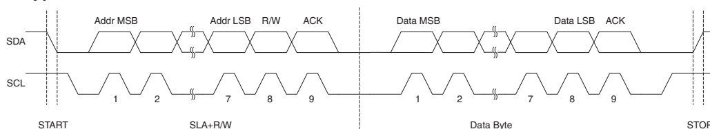
Figure 20-6. Typical Data Transmission
