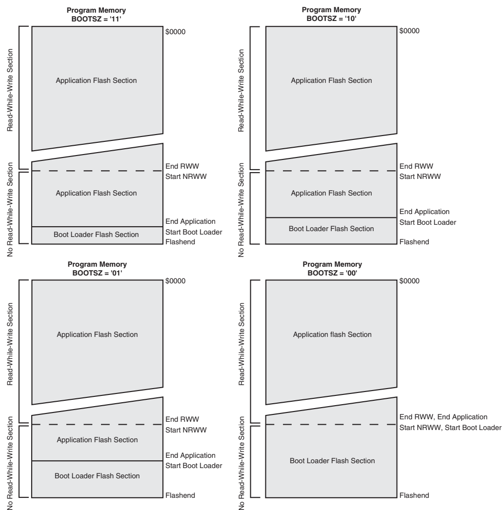
Figure 25-2. Memory Sections (1)
