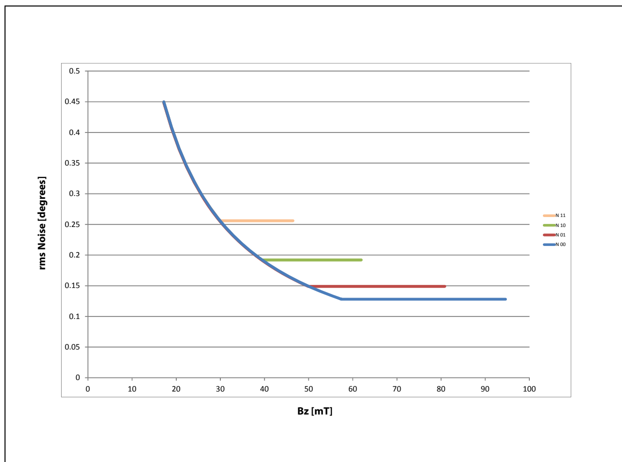
Figure 9: Worst Case Noise Performance of the AS5050A
