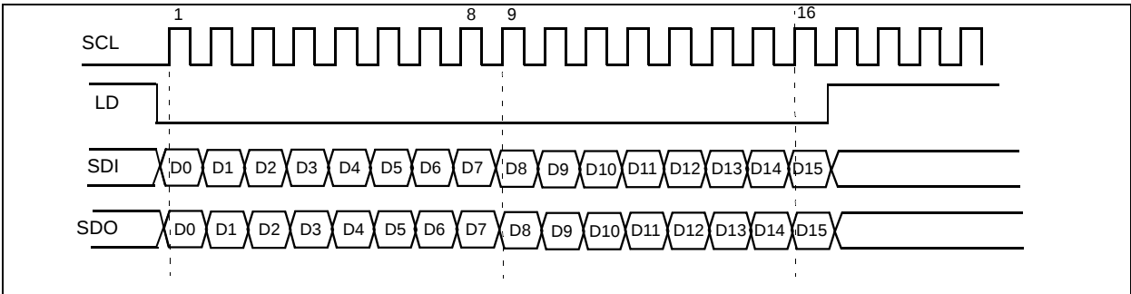
Figure 17. Write operation
