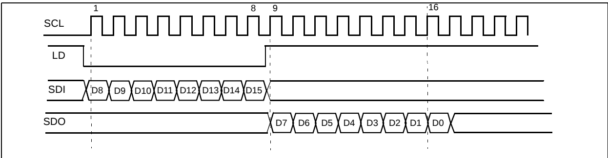
Figure 18. Read operation
