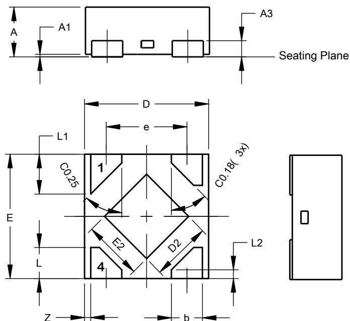
X2-DFN1010-4
