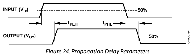
Figure 24. Propagation Delay Parameters
