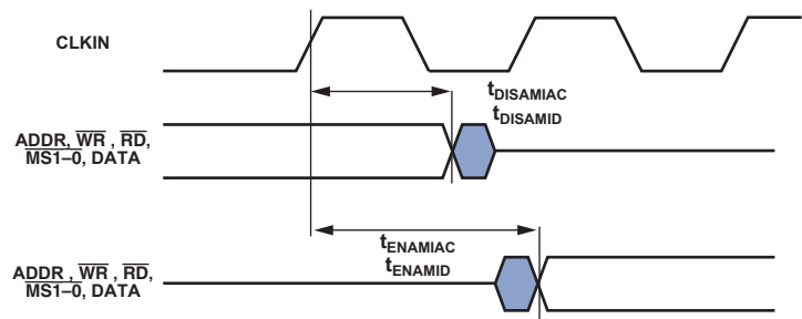
Figure 20. AMI Enable/Disable
