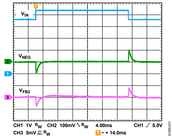
Figure 32. Inverting Regulator Line Transient, V_{IN} = 4.5\text{ V} to 5.5\text{ V} Step, V_{NEG} = -15\text{ V} , R_{LOAD2} = 300\ \Omega , f_{SW} = 2.4\text{ MHz} , T_A = 25^\circ\text{C}
