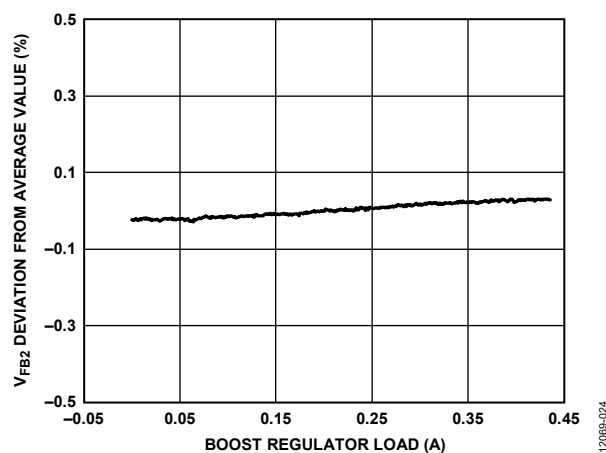
Figure 25. Cross Regulation, Inverting Regulator V_{FB2} Regulation over Boost Regulator Current Load, V_{IN} = 5V , V_{POS} = 15V , V_{NEG} = -15V , f_{SW} = 2.4MHz , T_A = 25^\circ C , Inverting Regulator Run in Continuous Conduction Mode with Fixed Load for Test
