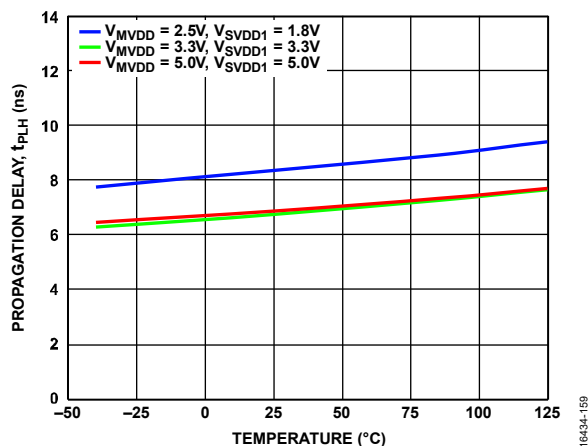
Figure 54. SPI Channels Propagation Delay ( t_{PLH} ) vs. Temperature at Various Supply Voltages
