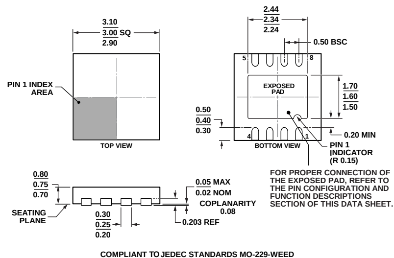
Figure 73. 8-Lead Lead Frame Chip Scale Package [LFCSP_WD] 3 mm × 3 mm Body, Very Very Thin, Dual Lead (CP-8-11)
