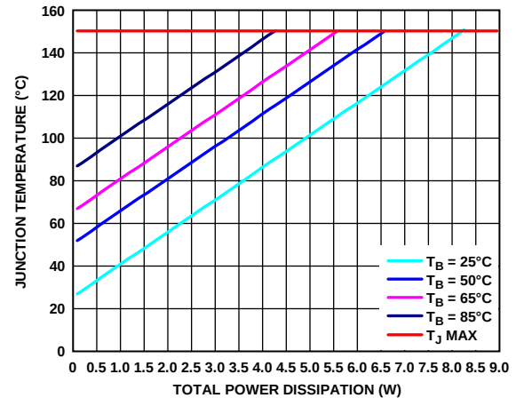
Figure 61. Junction Temperature vs. Total Power Dissipation for the 8-Lead LFCSP
