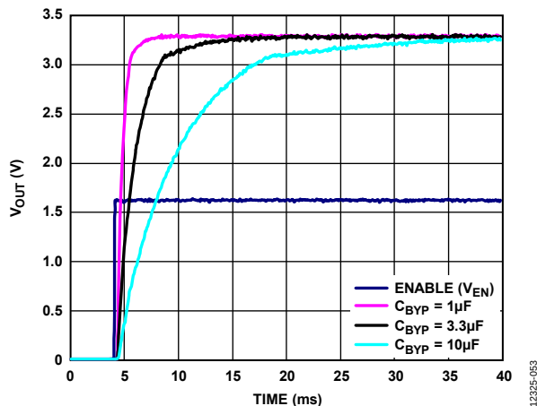
Figure 54. Typical Start-Up Behavior with C_{BYP} = 1 \mu F to 10 \mu F
