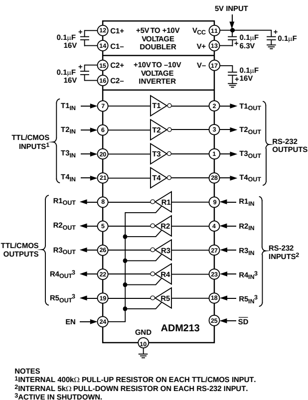
Figure 11. ADM213 Typical Operating Circuit
