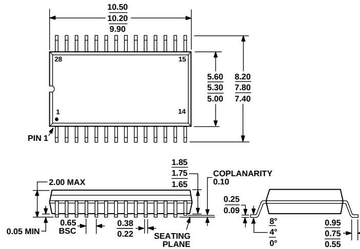
Figure 27. 28-Lead Shrink Small Outline Package [SSOP] (RS-28) Dimensions shown in millimeters
