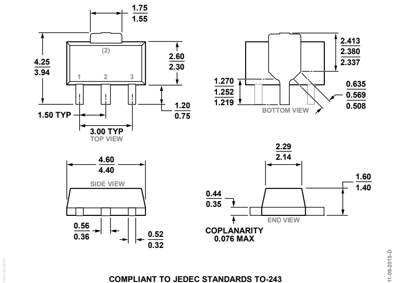
COMPLIANT TO JEDEC STANDARDS TO-243 Figure 33. 3-Lead Small Outline Transistor Package [SOT-89] (RK-3) Dimensions shown in millimeters
