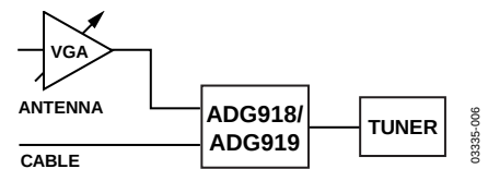
Figure 28. Tuner Modules
