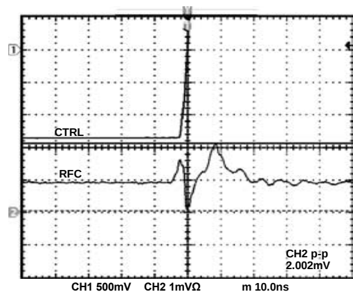
Figure 16. Video Feedthrough
