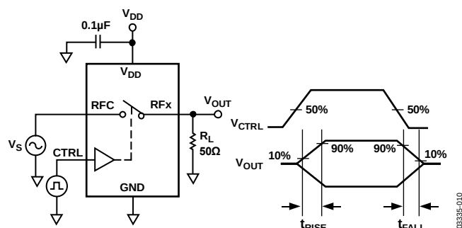
Figure 20. Switch
