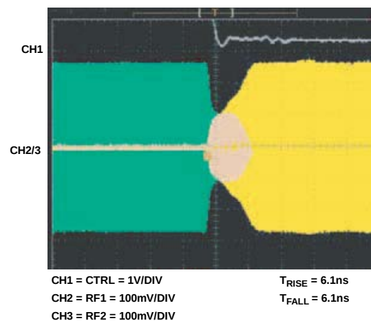
Figure 15. Switch Timing
