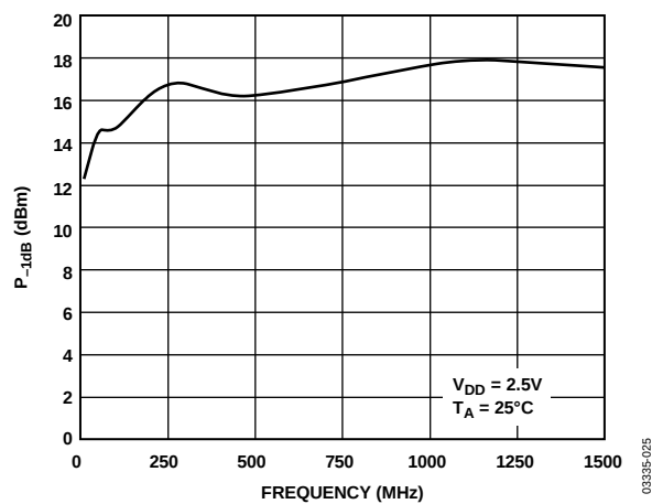
Figure 18. P_{-1dB} vs. Frequency
