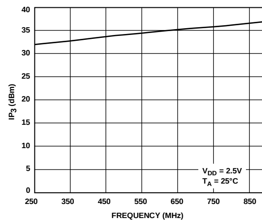
Figure 17. IP3 vs. Frequency
