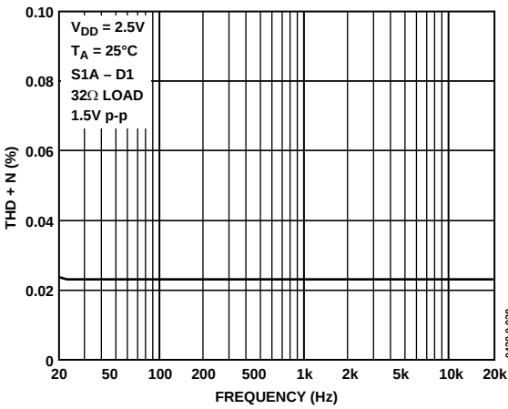
Figure 17. Total Harmonic Distortion + Noise
