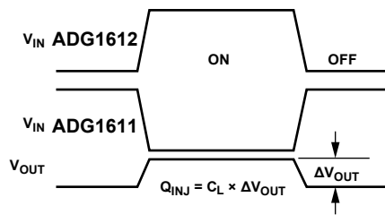
Figure 33. Charge Injection
