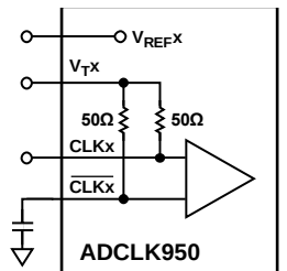
Figure 23. DC-Coupled 3.3 V CMOS Input Termination
