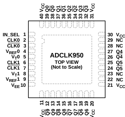
Figure 2. Pin Configuration
